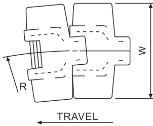
880 (Side Flexing Plastic Chain)
